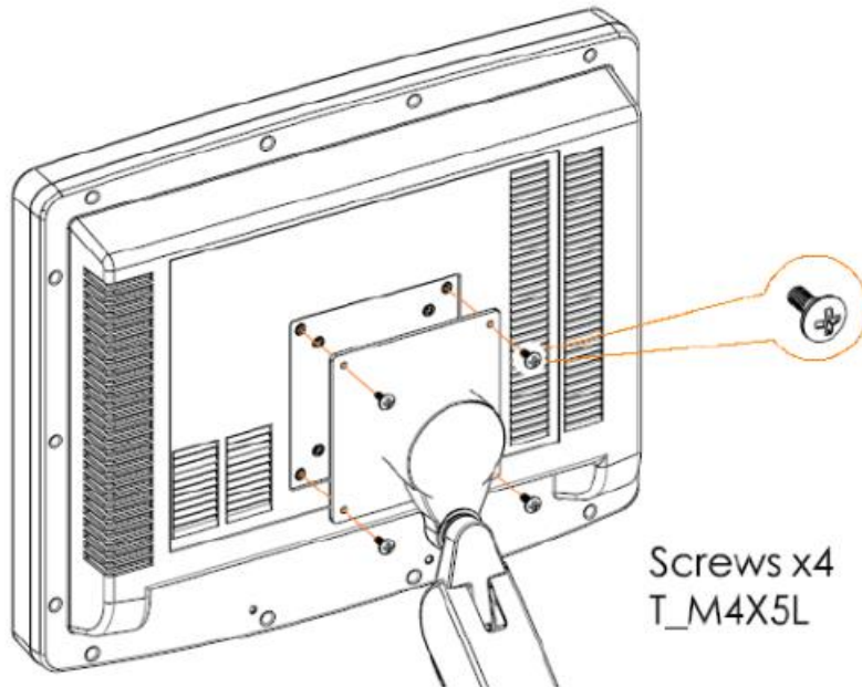
Figure 26 ARCHMI-9xxB Series VESA Mounting
