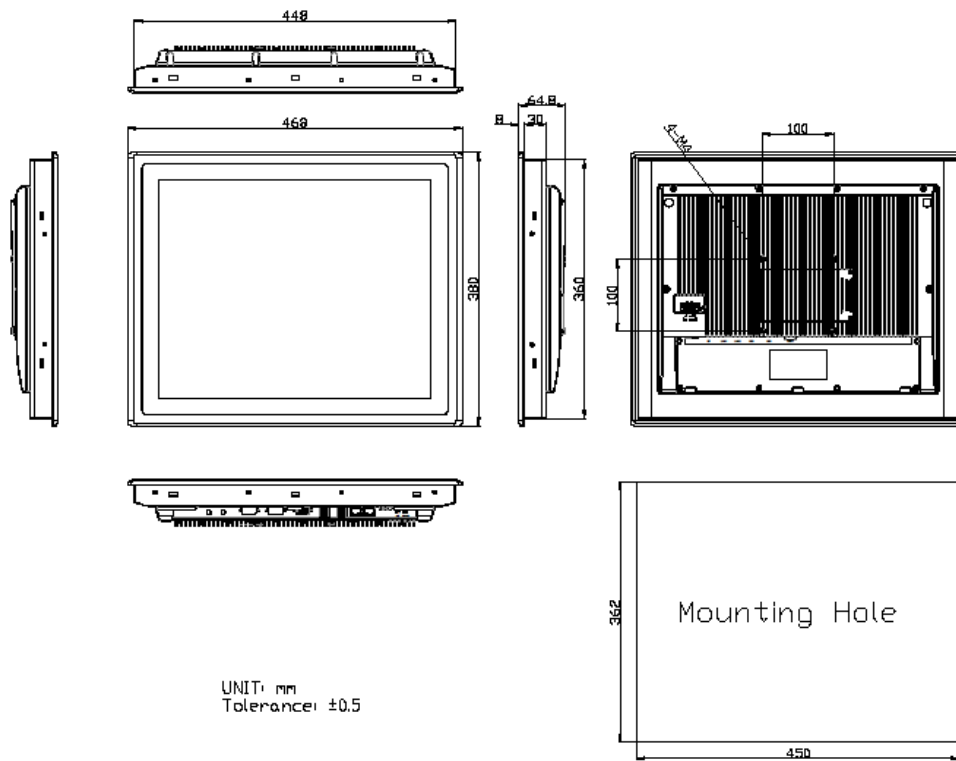
Figure 7 Dimensions of ARCHMI-919BP/BR (H)
