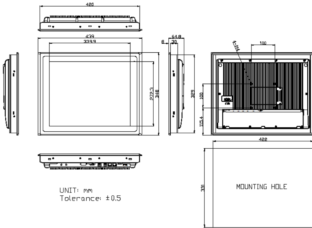
Figure 5 Dimensions of ARCHMI-917BP/BR (H)
