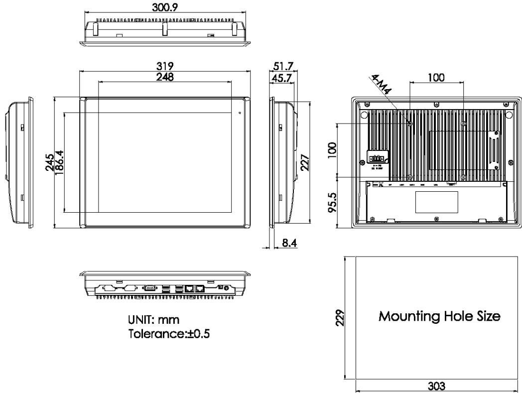
Figure 1 Dimensions of ARCHMI-912BP/BR (H)
