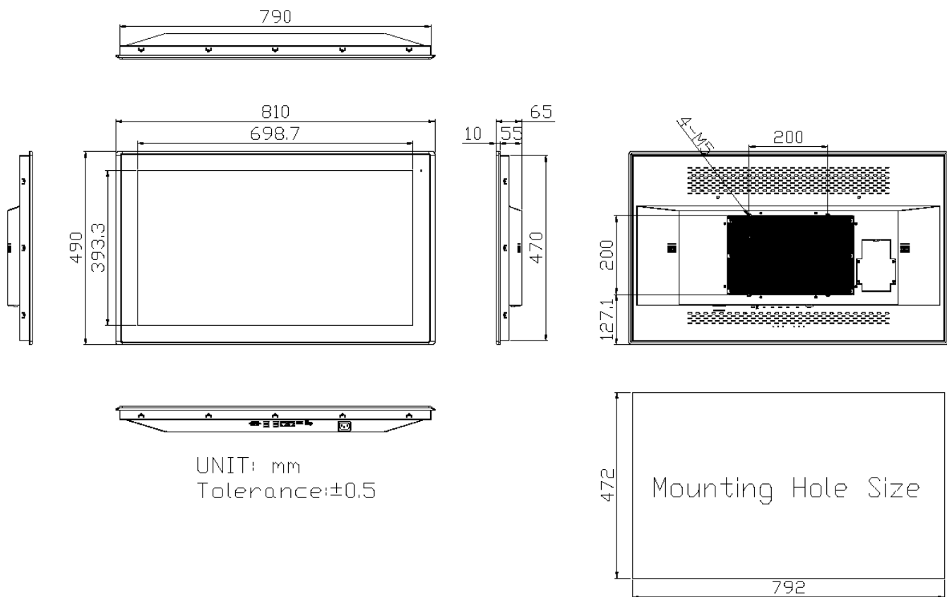
Figure 9 Dimensions of ARCHMI-932BP
