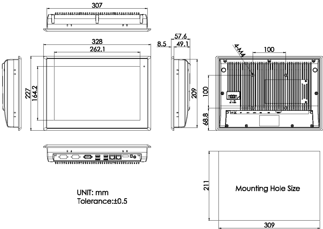
Figure 2 Dimensions of ARCHMI-912WBP/WBR (H)
