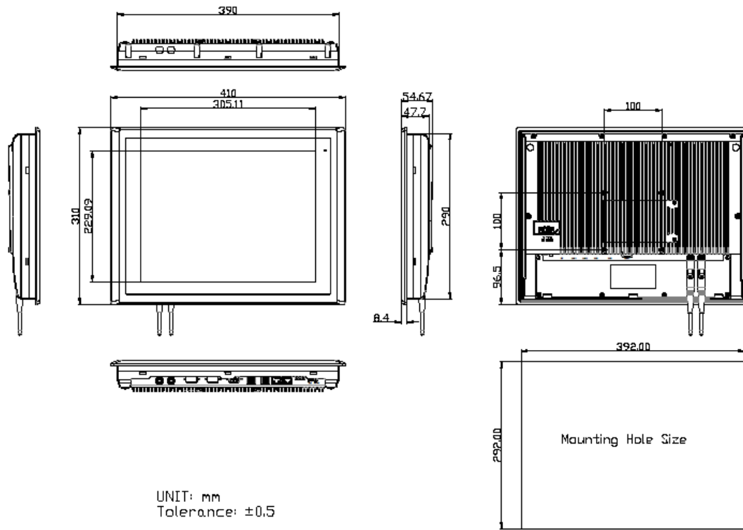
Figure 3 Dimensions of ARCHMI-915BP/BR (H)
